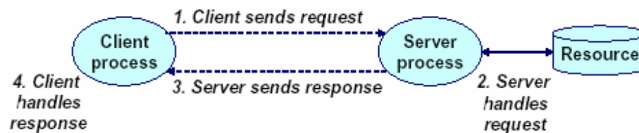
Gambar 9.1 Transaksi Client – server
