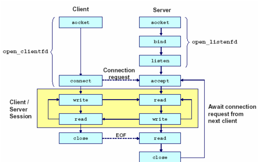
Gambar 9.4 Ilustrasi Interface socket
